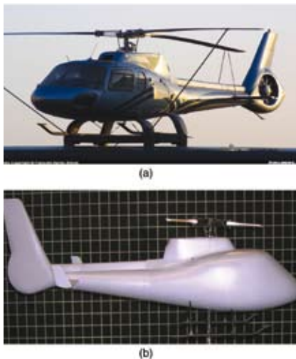
Figure 1(a) Eurocopter 350Z Helicopter Prototype (b) A generic 350Z model with 1:7.126 scaled-down
