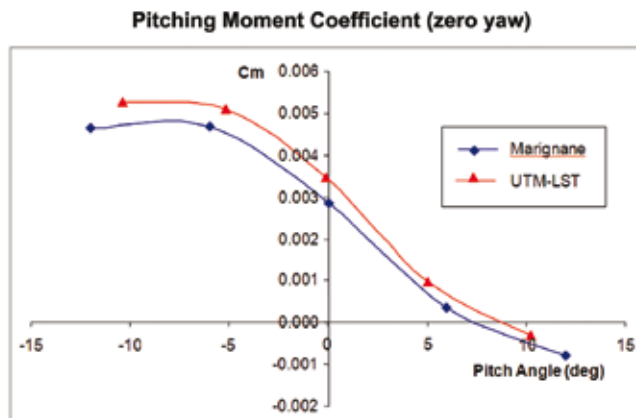
Figure 6: Pitching moment coefficient at zero yaw
