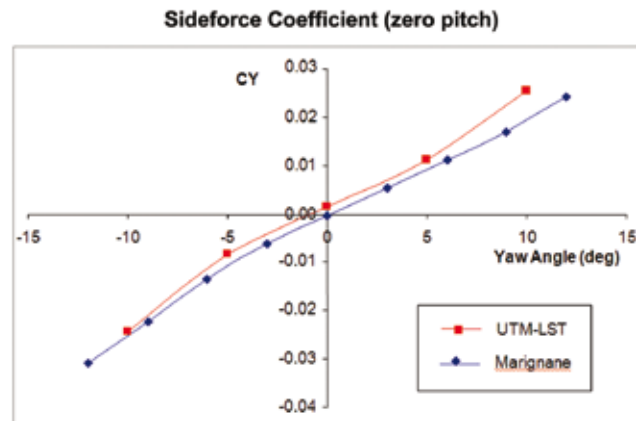
Figure 5: Sideforce coefficient at zero pitch
